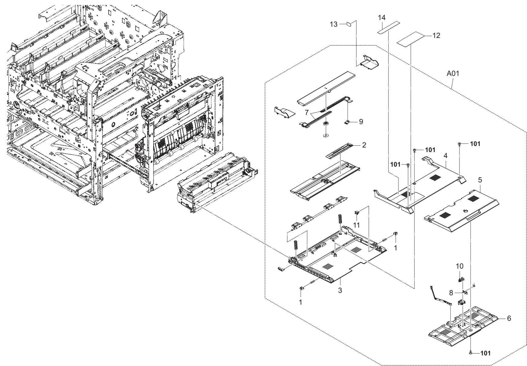
FIG. 10 Paper Conveying Section 3
