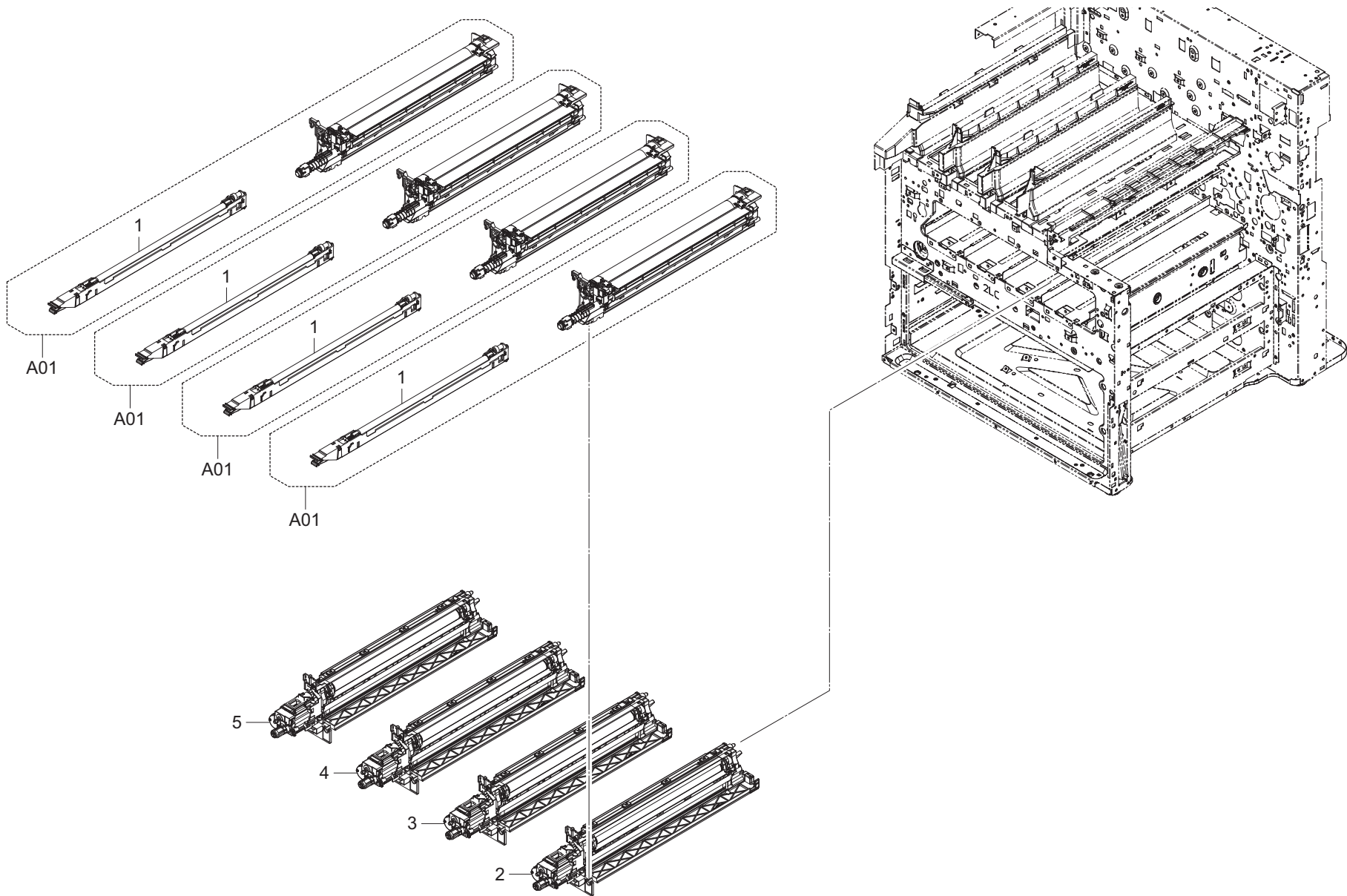
FIG. 13 Image Formation & Developer Section
