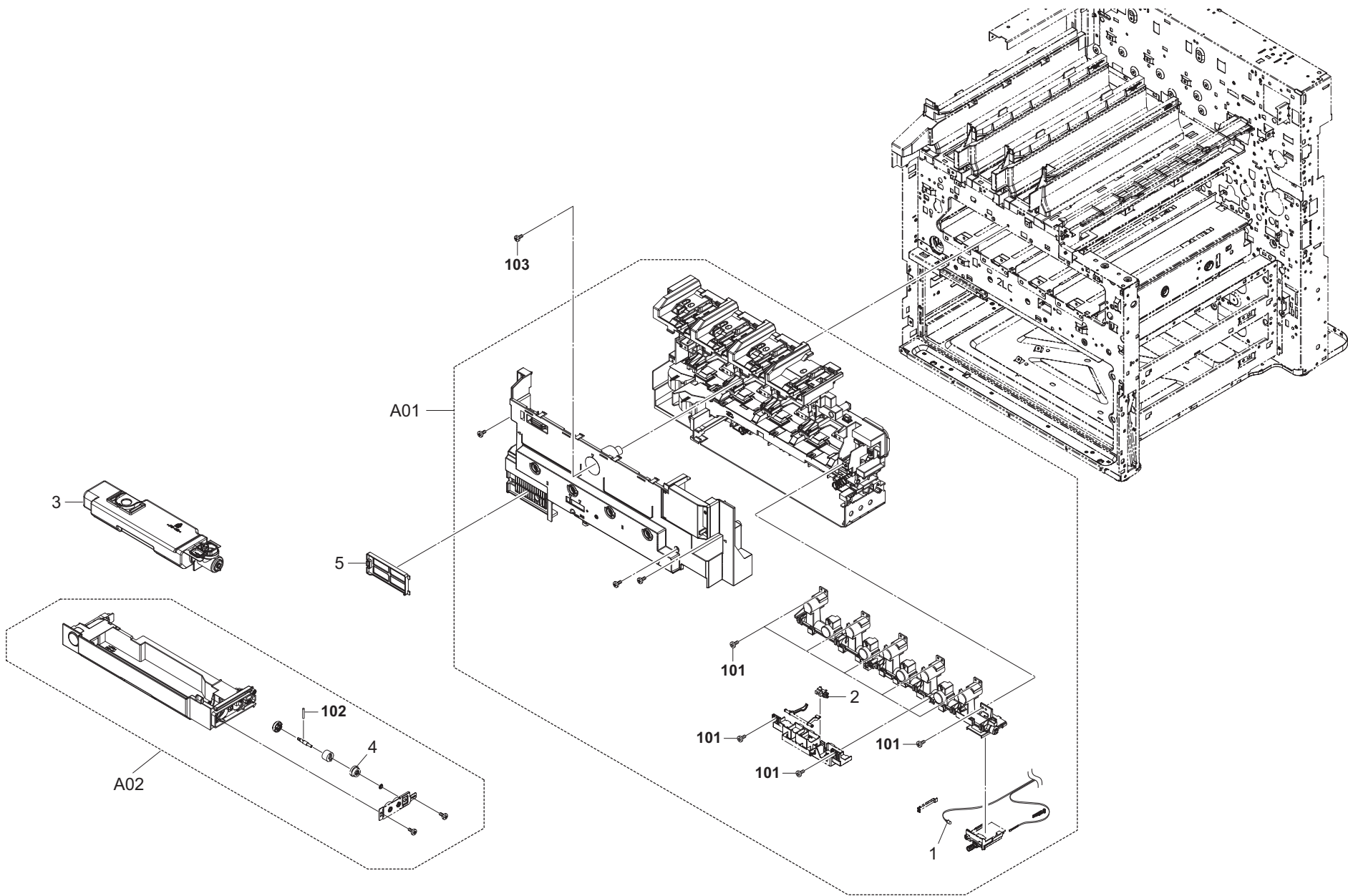
FIG. 14 Inner Section
