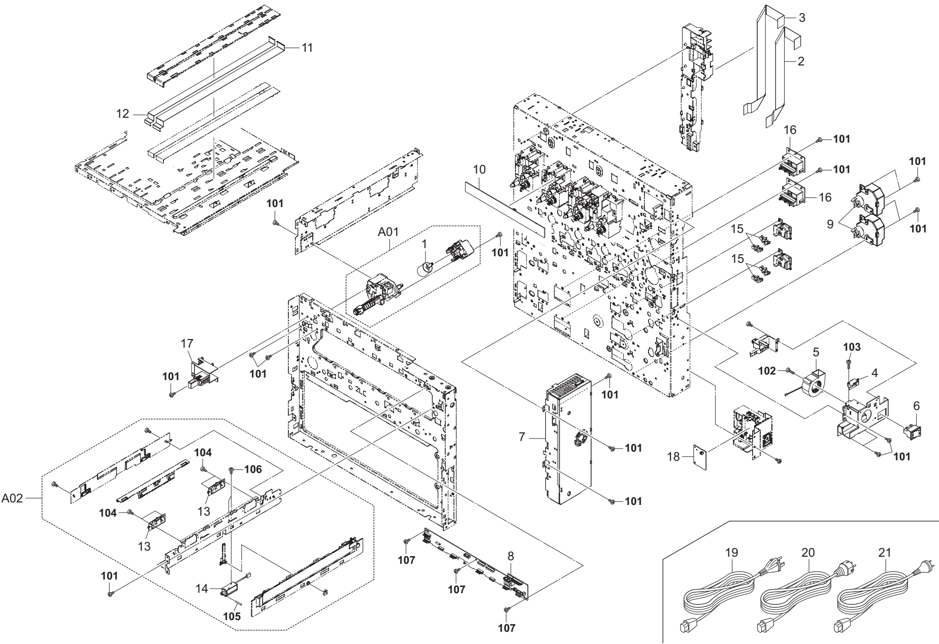
FIG. 21 Electrical Components 1
