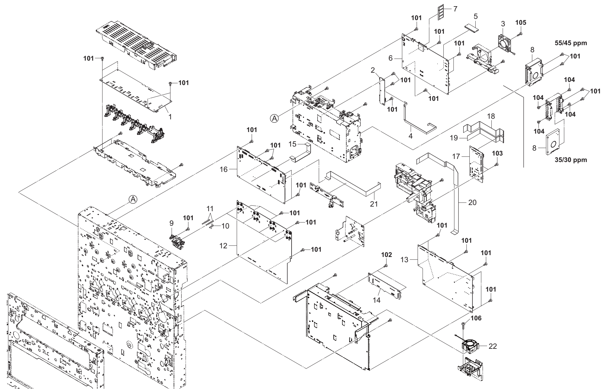
FIG. 22 Electrical Components 2
