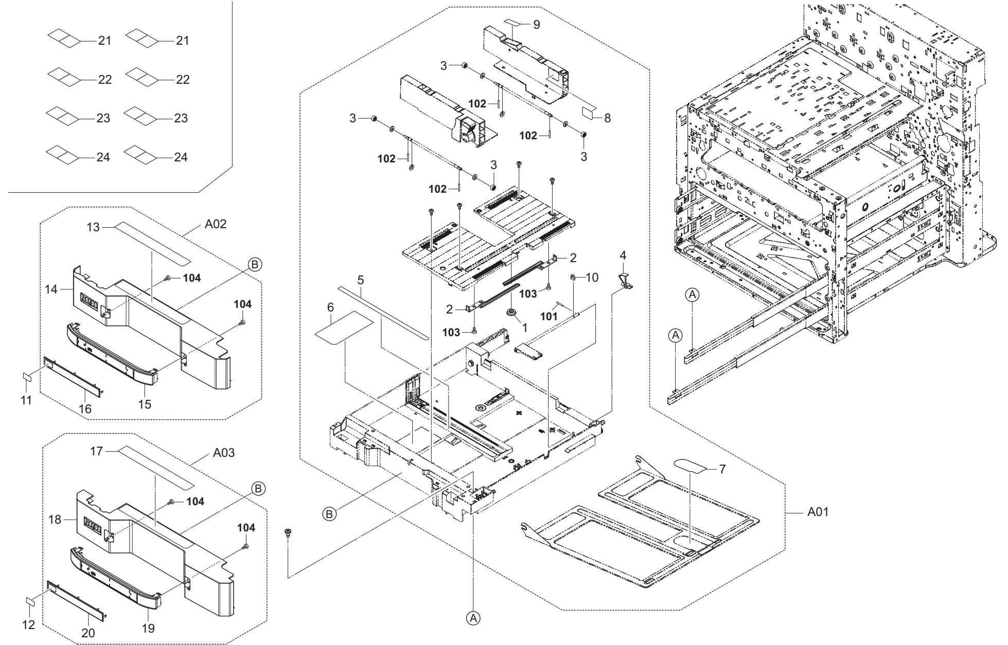
FIG. 5 Paper Cassettes
