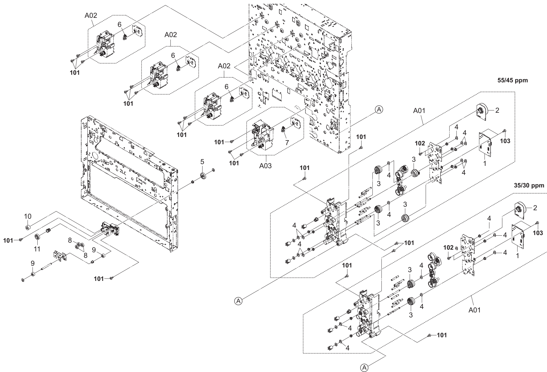
FIG. 18 Drive Section 2
