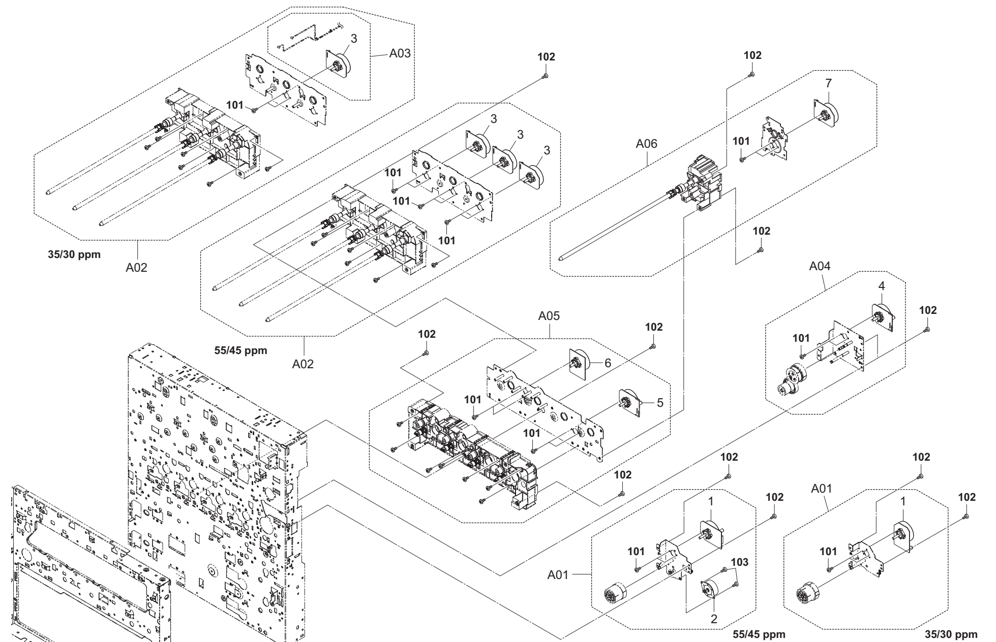
FIG. 17 Drive Section 1
