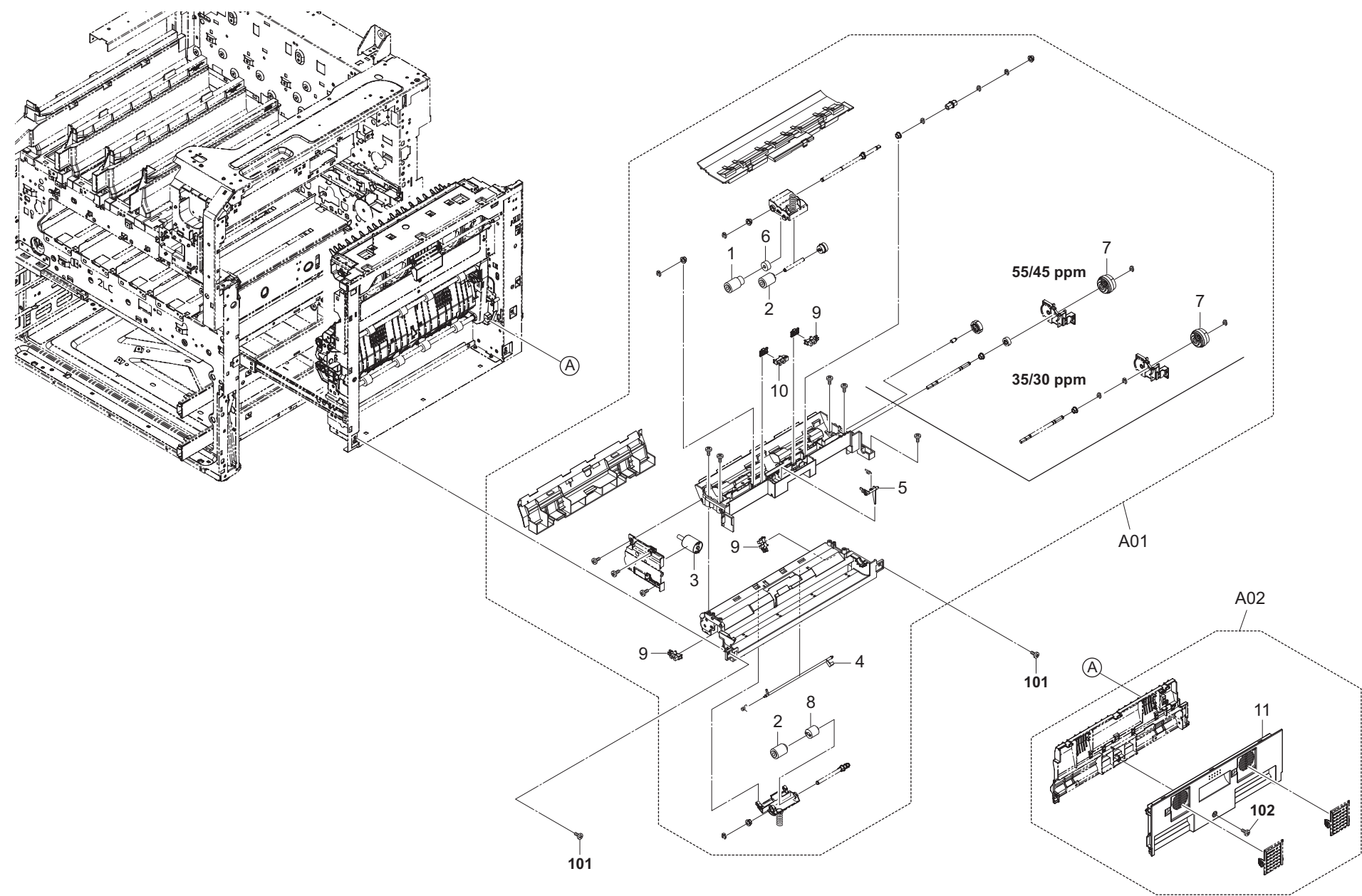
FIG. 9 Paper Conveying Section 2
