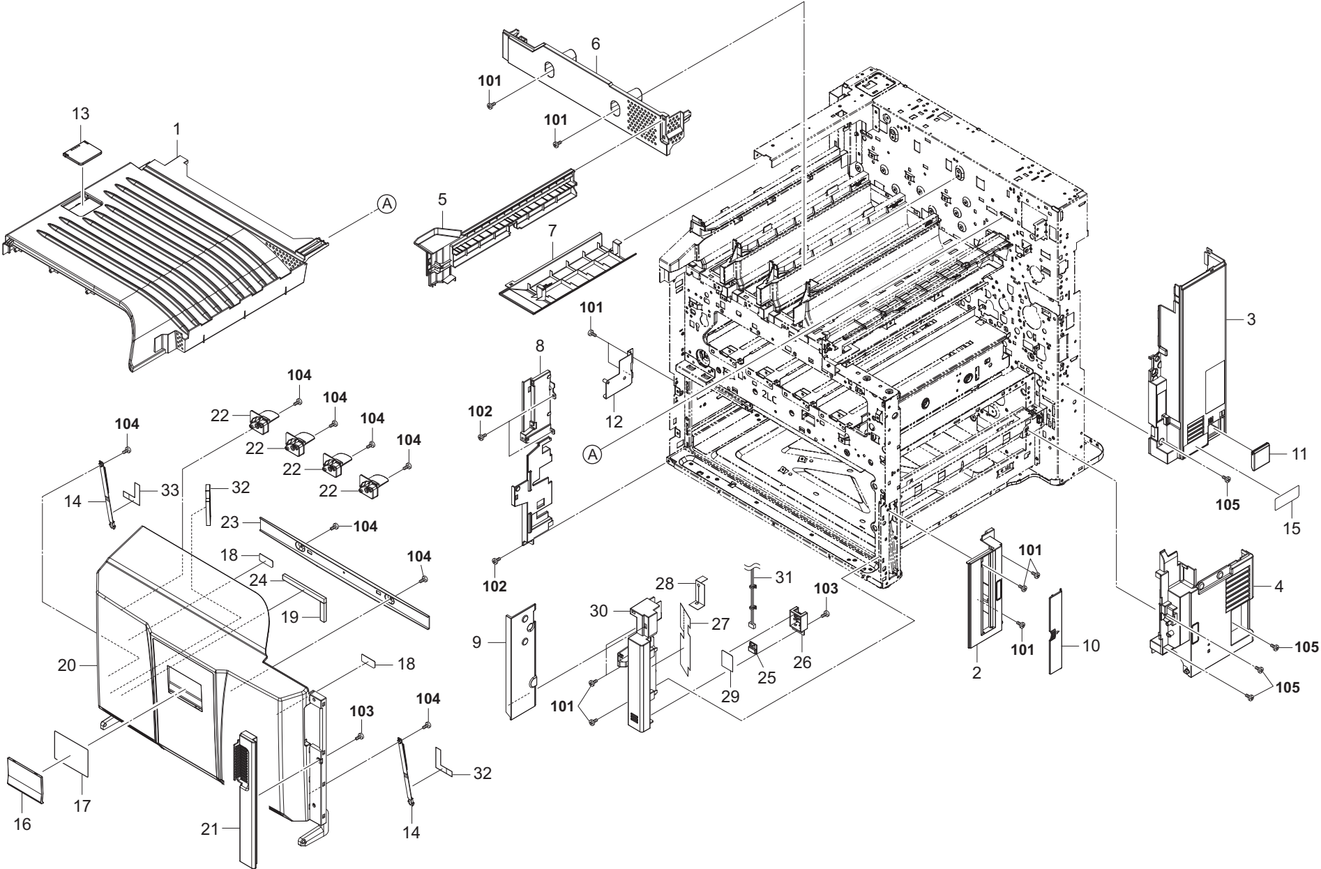
FIG. 1 Covers 1
