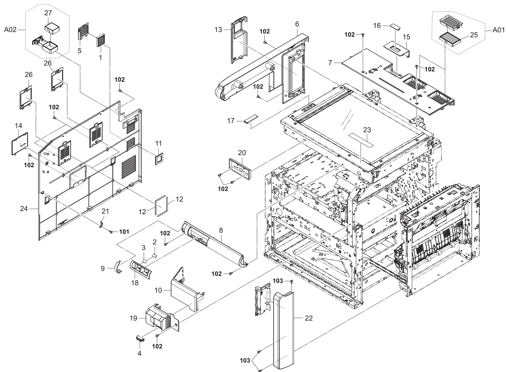
FIG. 2 Covers 2
